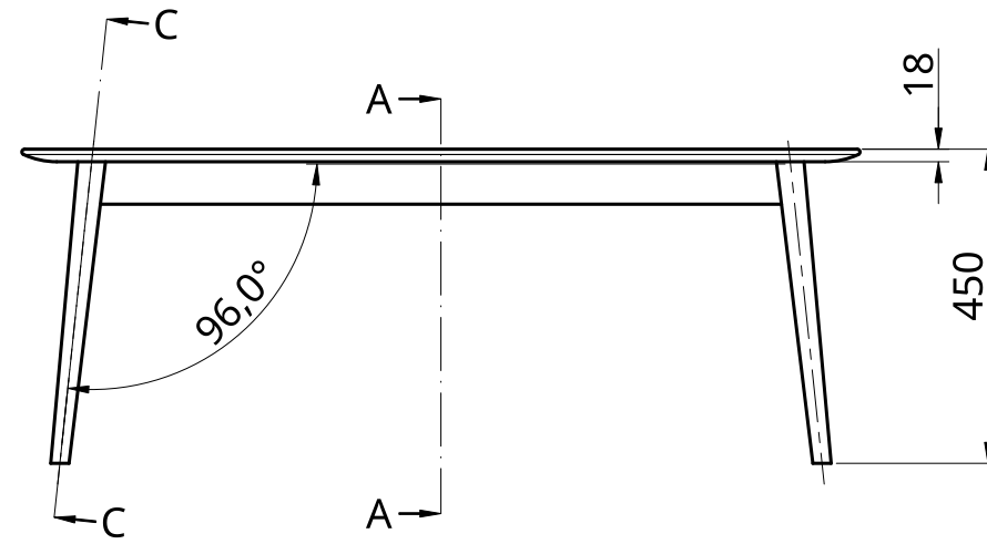
Front
